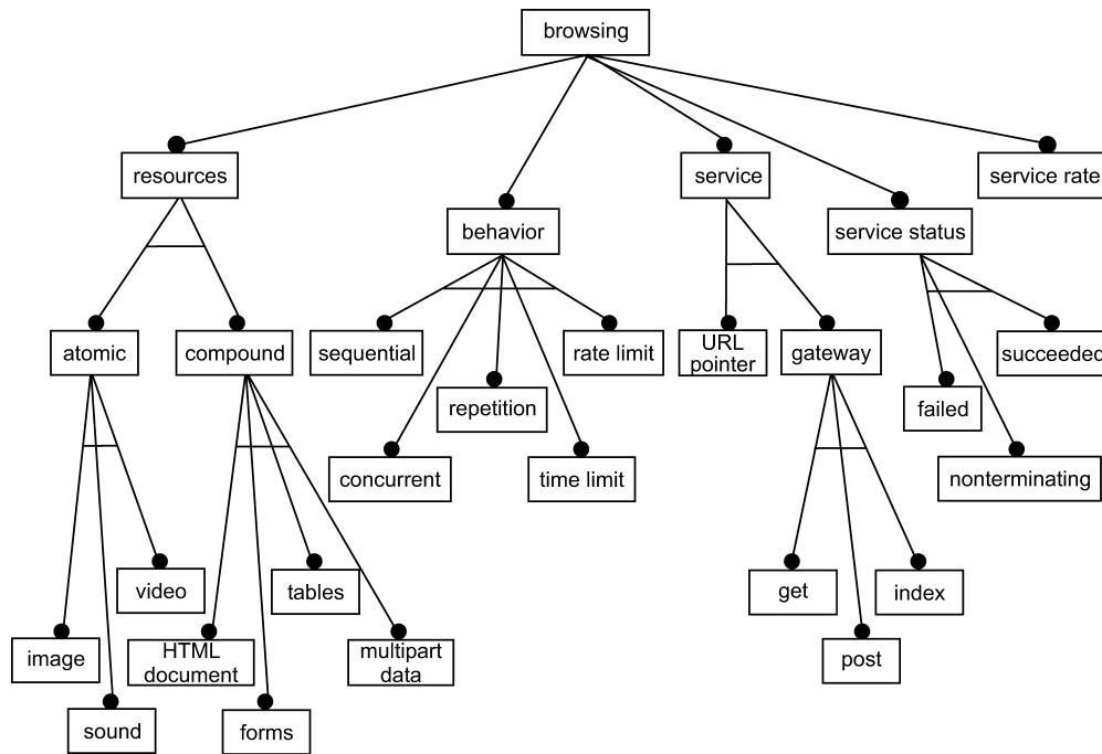
Fig. 1. Feature diagram for Web browsing.
