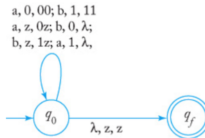
Linz Fig. 7.3: Transition Graph for Example 7.4
