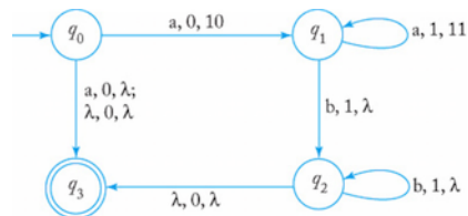
Linz Fig. 7.2: Transition Graph for Example 7.2
